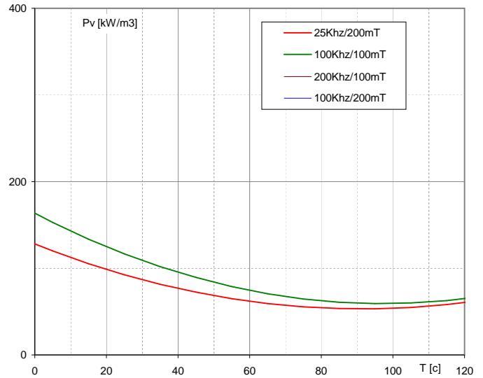
Specific Power Loss vs Temperature
