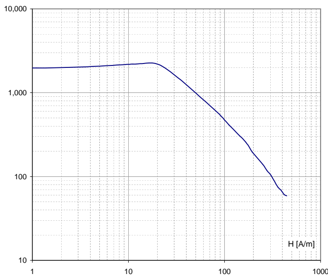
Permeability vs Magnetic Field Strength
