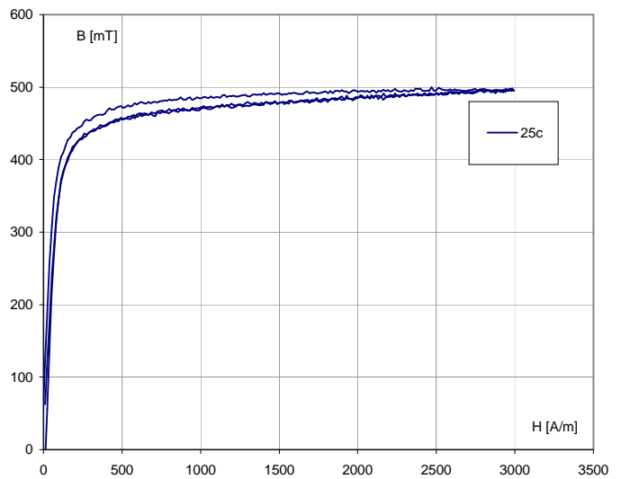
B-H Loops
