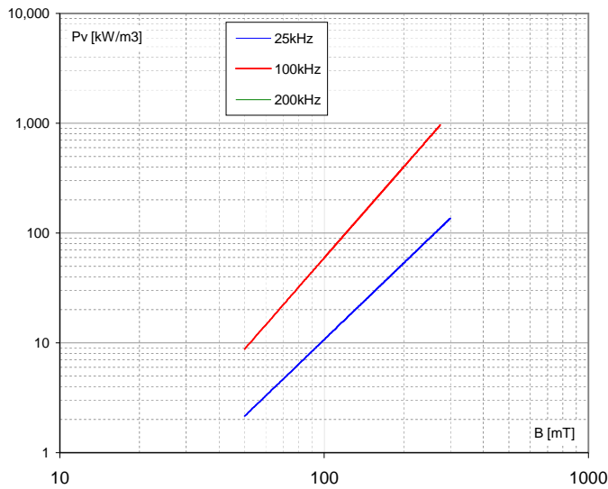
Specific Power Loss vs. Flux Density
